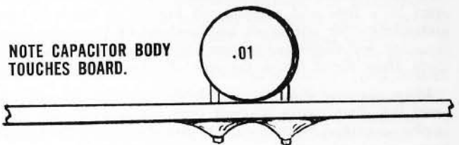
DETAIL "C"
